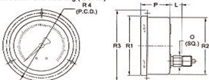
Back Conn. Penal Mounting (BCPM)
