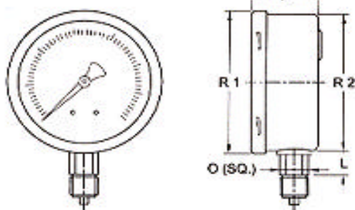
Bottom Connection Bracket Mounting (FB(BKT))
